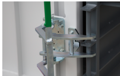
Bell-crank lever for quick and safe opening of the door
