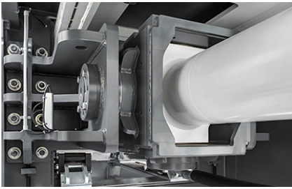
Gimballed press cylinder system - Reduced wear on the pressing cylinder and press ram guides
